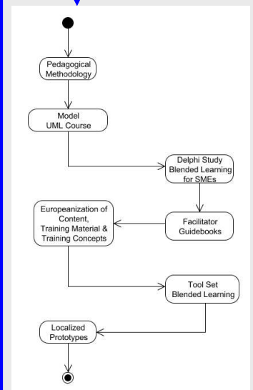
Figure 2: Up2UML Activities
